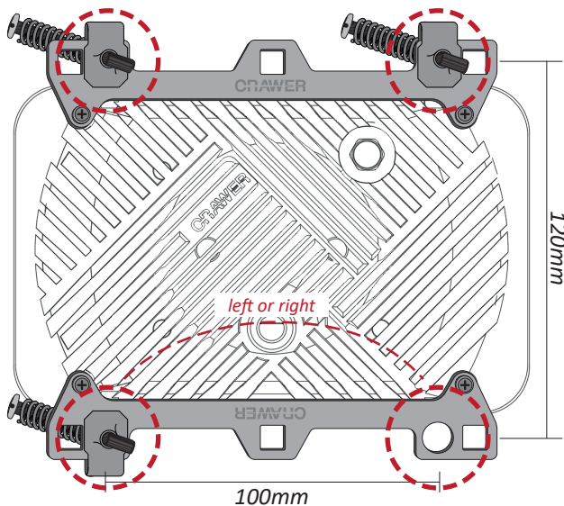
4x short screw
