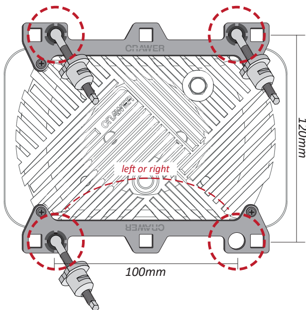
4x short screw
