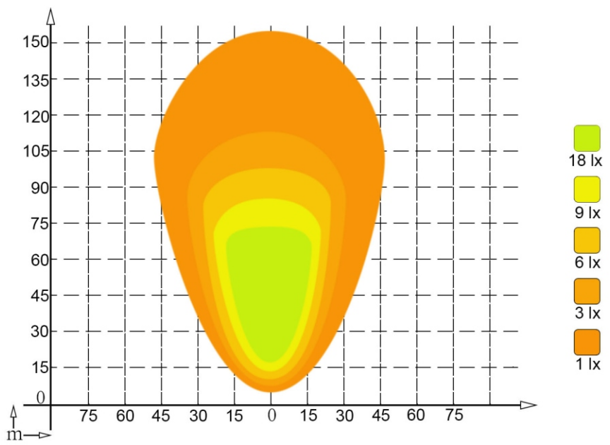
LOW BEAM PATTERN
